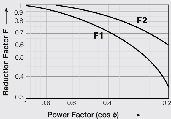
Reduction factor for ac inductive loads
