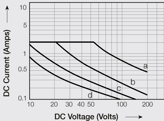
Maximum dc inductive load breaking capacity
