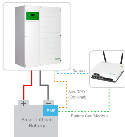
Lithium-ion battery with closed loop control
