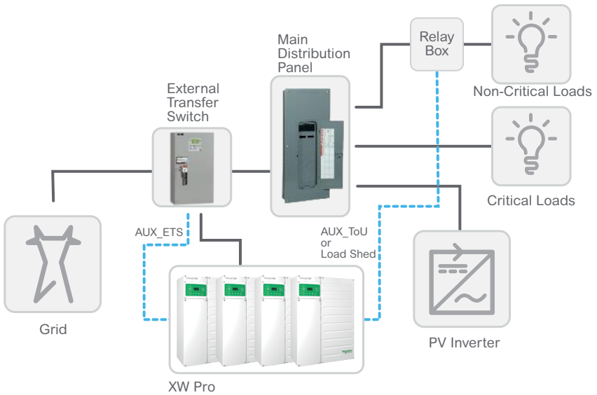
Example: External transfer and load shedding applications using XW Pro Aux in a system.
