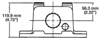
Top View
