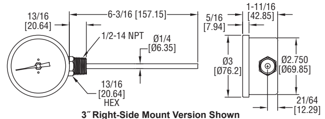
3" Right-Side Mount Version Shown
