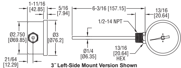
3" Left-Side Mount Version Shown
