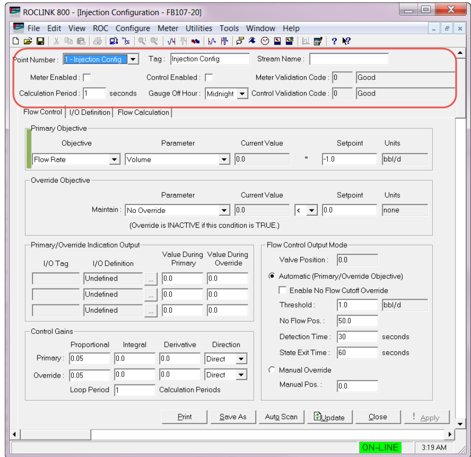
Figure 16. Injection Configuration – Main section (red box)
