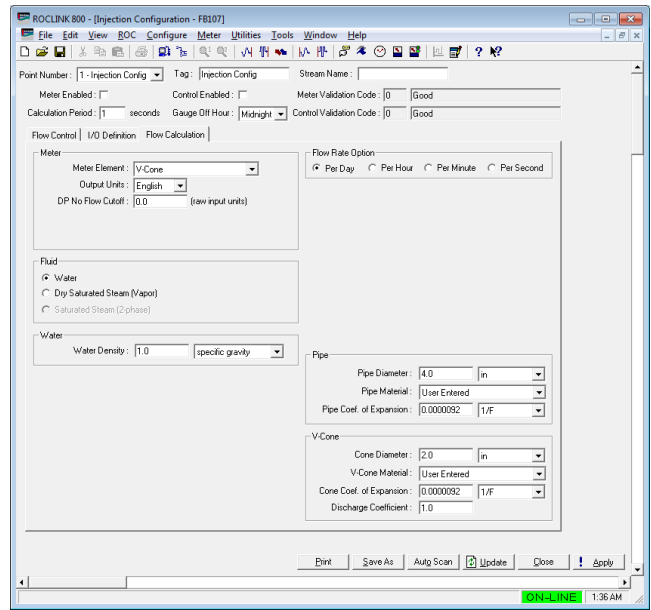
Figure 21. Injection Configuration – Flow Calculation Tab (Meter Element is set to V-Cone)
