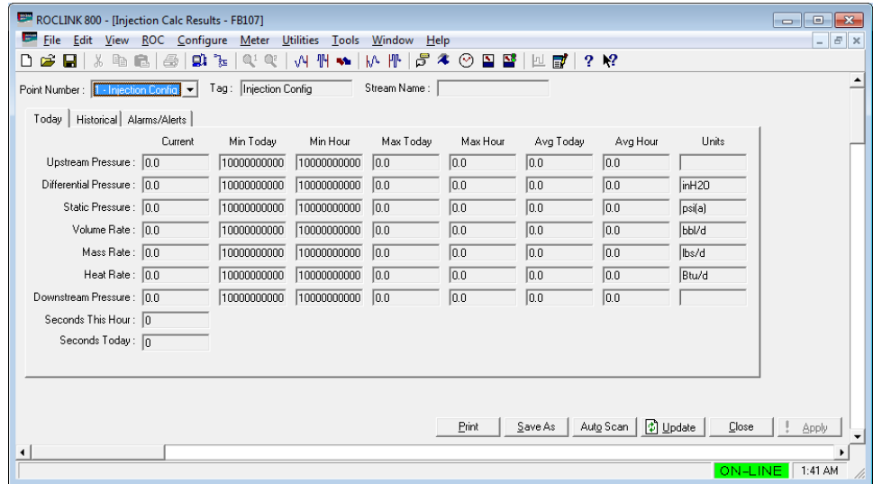
Figure 25. Injection Calc Results – Today tab
