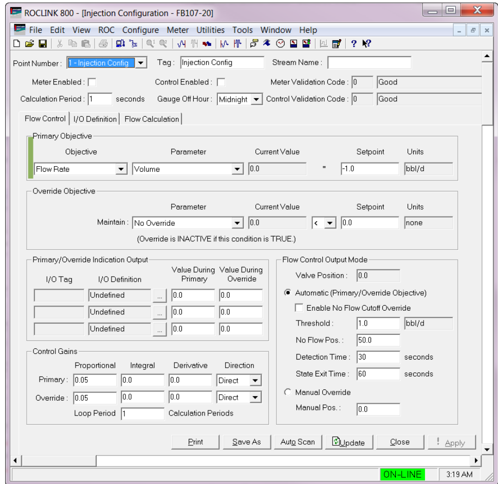
Figure 15. Injection Configuration Screen
