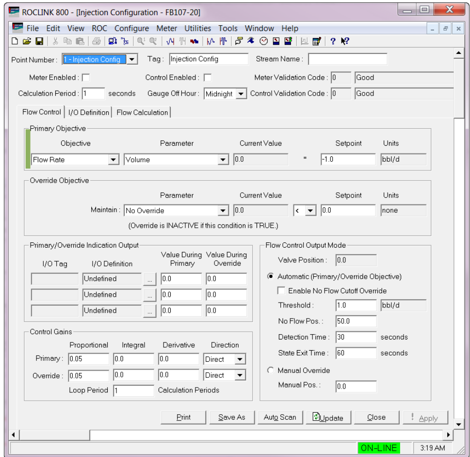
Figure 17. Injection Configuration – Flow Control Tab
