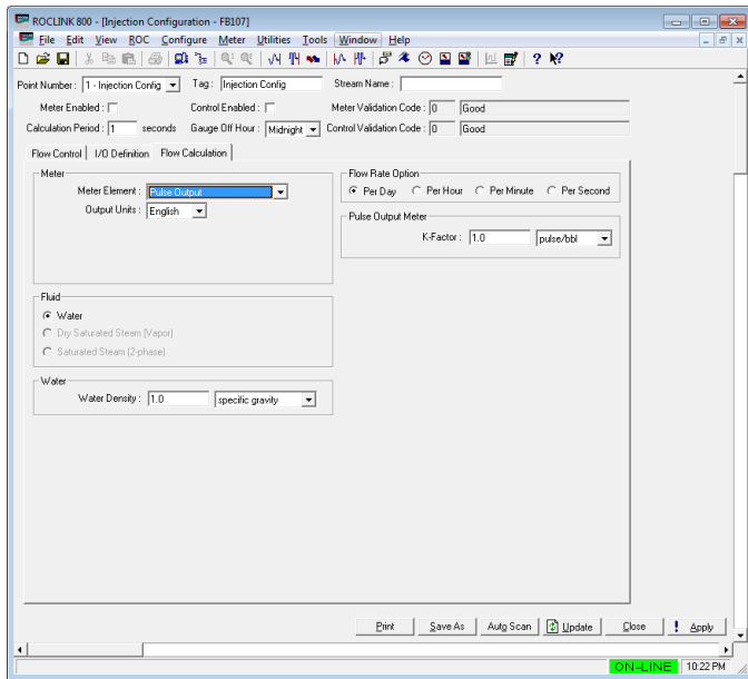
Figure 20. Injection Configuration – Flow Calculation Tab (Meter Element is set to Pulse Output)
