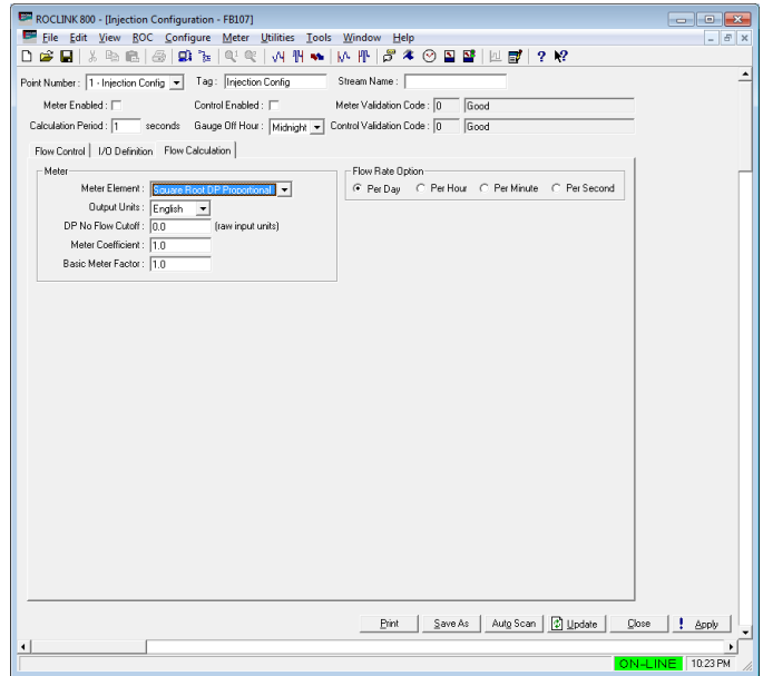
Figure 23. Injection Configuration – Flow Calculation Tab (Meter Element is set to Square Root DP Proportional)
