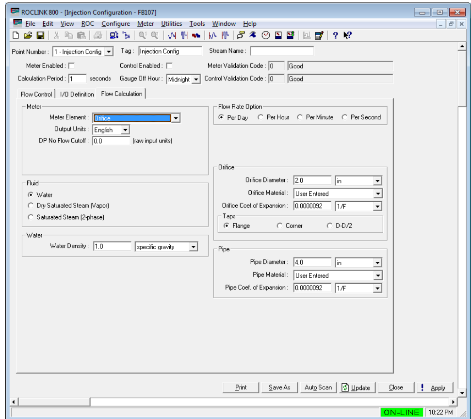
Figure 19. Injection Configuration – Flow Calculation Tab (Meter Element is set to Orifice)
