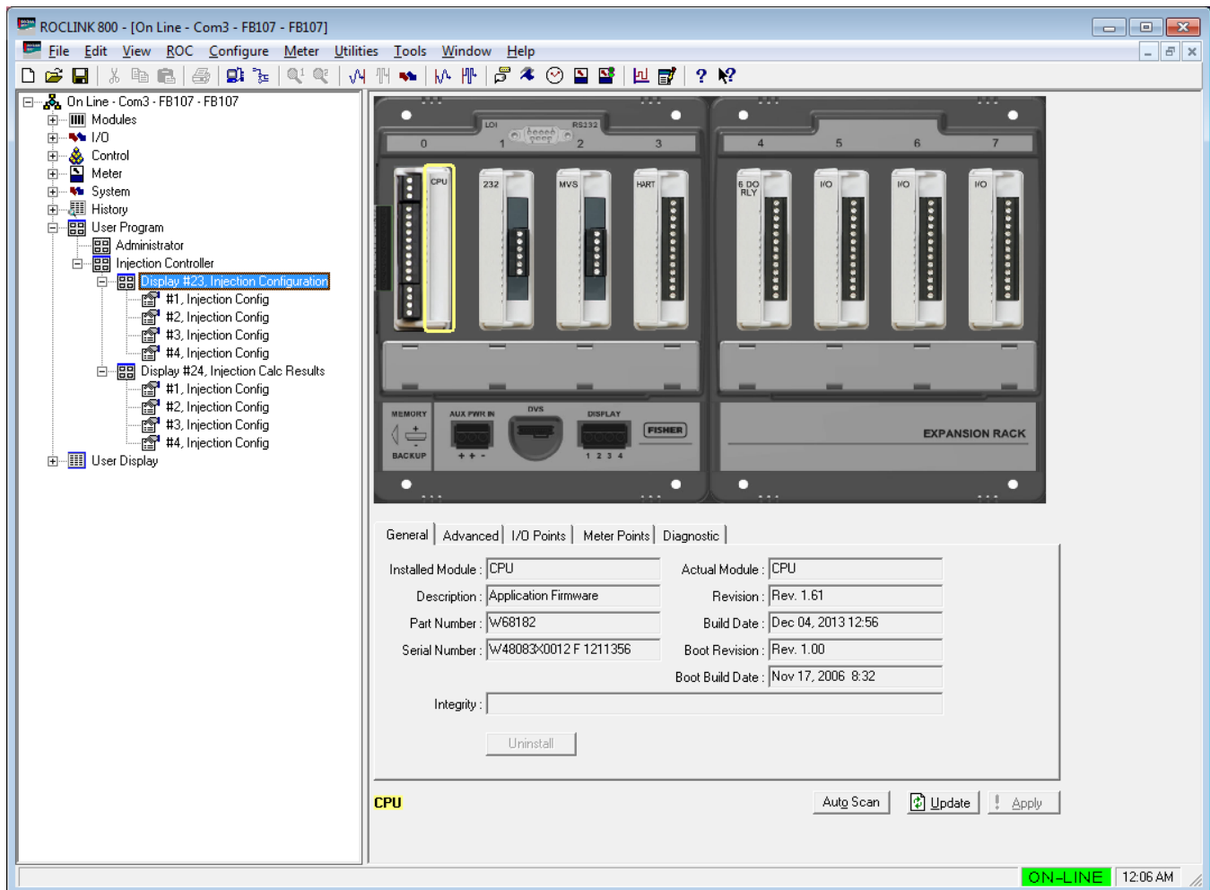
Figure 13. ROCLINK 800 for FB107
