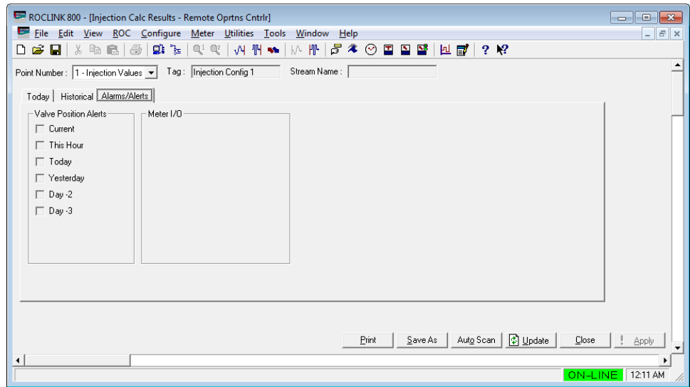
Figure 27. Injection Calc Results – Alarms/Alerts tab
